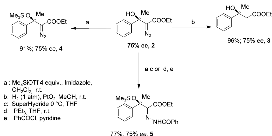
Scheme 2. Transformation of the diazo adducts occurred with no racemization.
