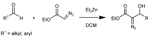
Scheme 1. Reaction of aldehydes in the presence of Et_2Zn as a base.
